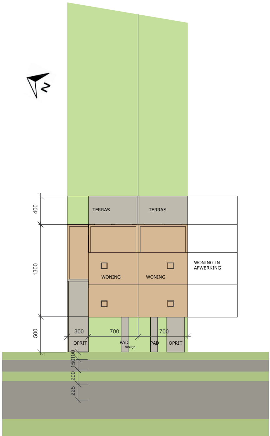
INPLANTINGSPLAN
